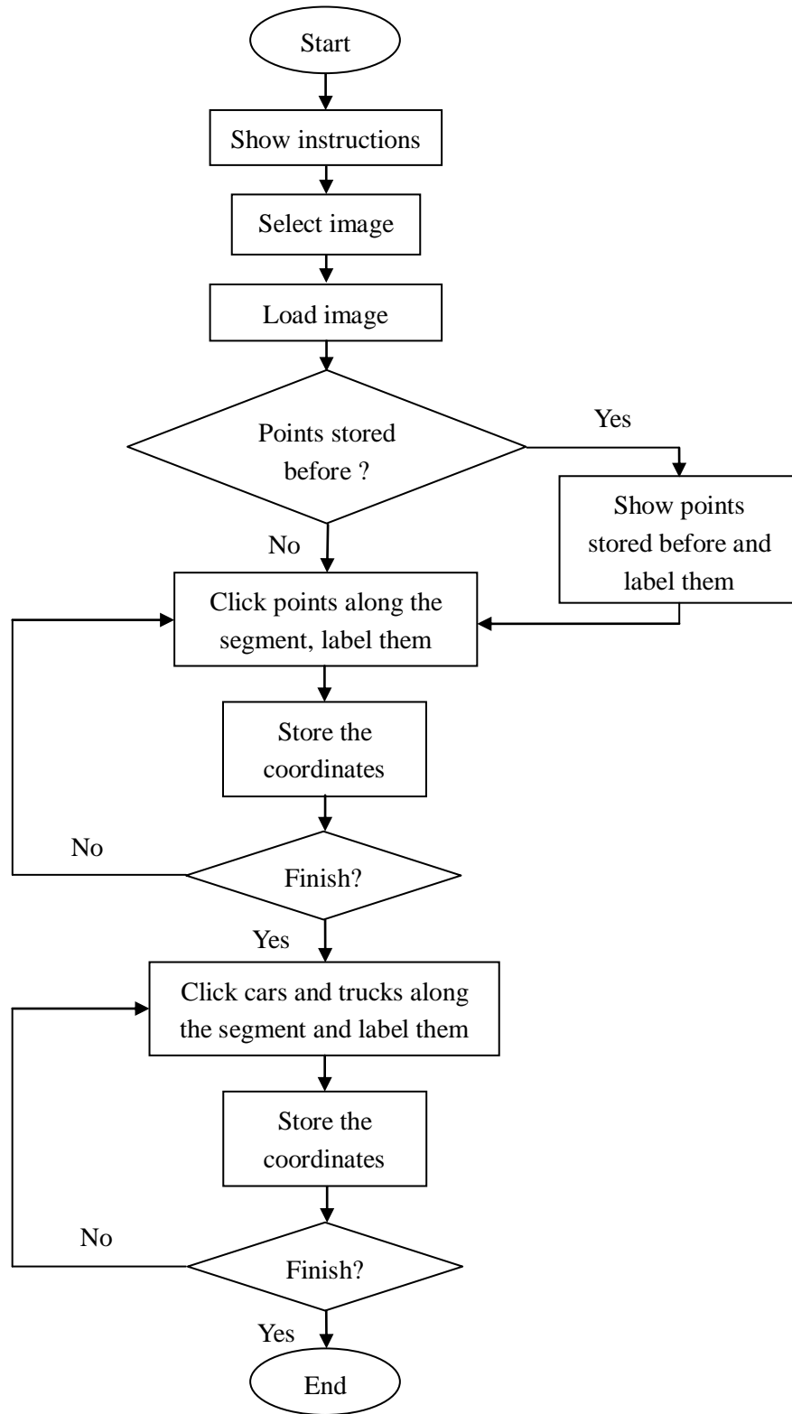
Figure 1. Flowchart of digitization program, digitizing.m
